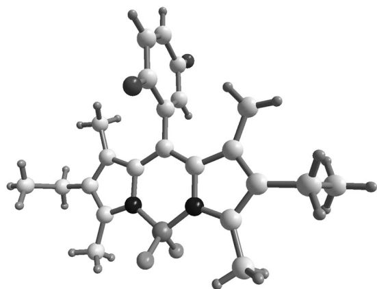
Figure 1. Molecular structure of the quinone derivative BD-Q.
