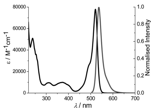
Figure 3. Typical absorption (black) and fluorescence (grey) spectra for BD-M in \text{CH}_3\text{CN} at room temperature.
