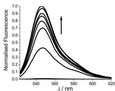
Figure 4. Observed increase in fluorescence intensity upon fixed-potential reduction of BD-PQ ( c \approx 4 \mu\text{M} ) in DCM (0.2 M TBATFB) using a conventional OTTLE cell.
