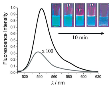
Figure 5. Fluorescence spectra recorded at 25 °C for BD-PHQ ( c \approx 4 \mu\text{M} ) in distilled water containing Triton-X (5% v/v) and \text{Na}_2\text{HPO}_4 (0.18 M), before (dark line) and after (grey line) the addition of \text{Na}_2\text{CO}_3 \cdot \text{H}_2\text{O}_2 . Excitation wavelength \lambda = 495 \text{ nm} . Insert shows a cuvette illuminated with a standard UV-lamp, and the changes in fluorescence over time during oxidation by peroxide.
