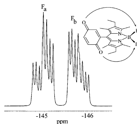
Figure 2. ^{19}\text{F} NMR spectrum recorded for BD-Q in \text{CDCl}_3 showing the coupling patterns and tentative assignment.
