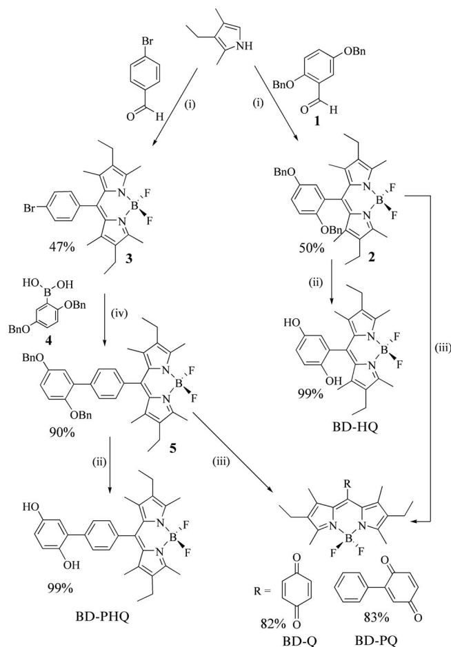
Scheme 1. Reagents and conditions. (i) DCM, TFA, room temp.; DDQ; N,N -diisopropylethylamine, \text{BF}_3 \cdot \text{Et}_2\text{O} . (ii) \text{H}_2 , 4 atm, DCM/MeOH, Pd/C (10%). (iii) \text{H}_2 , 4 atm, DCM/MeOH, Pd/C (10%); DDQ, THF.
